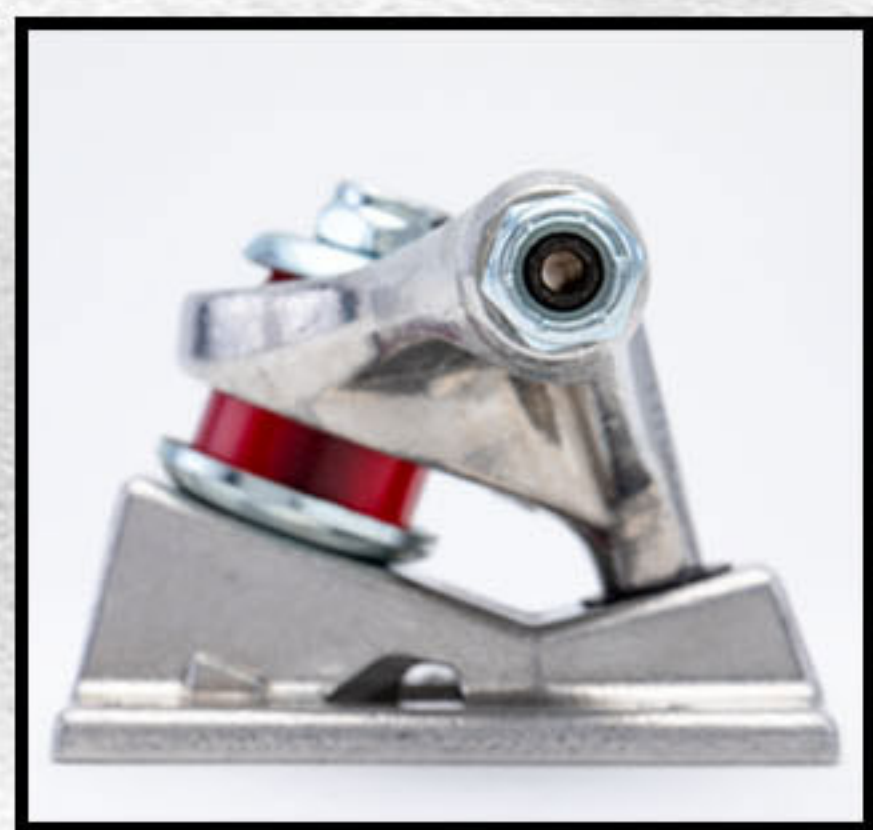
HOLLOW AXLE
